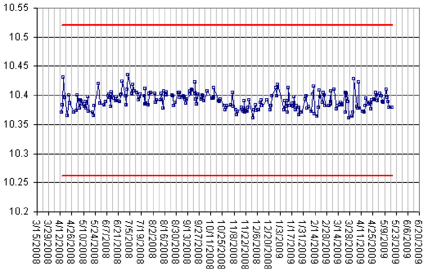
Measured Sensitivity @ F_{ref} (mV/m/s 2 )
