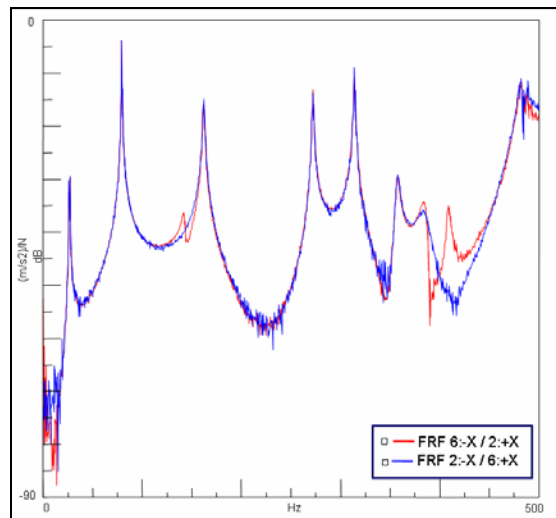
Figure 4. Reciprocity Measurement for MIMO Test
