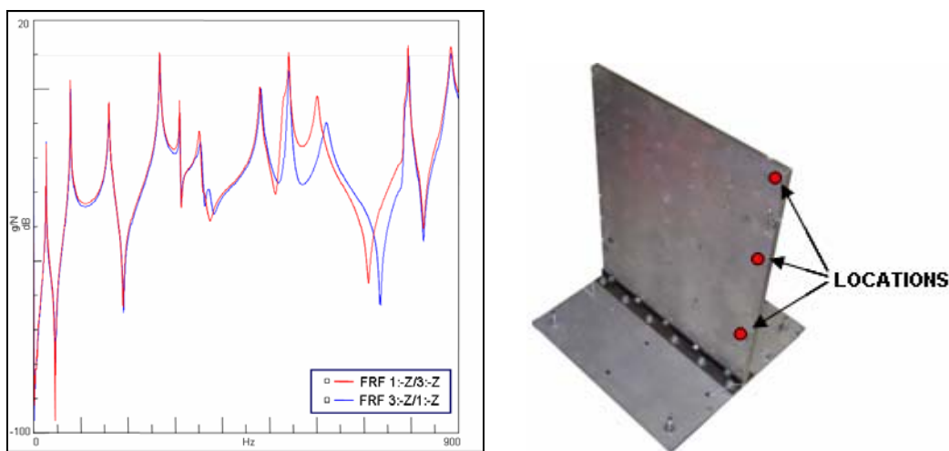
Figure 5. Reciprocity Measurement between Upper and Lower SISO Measurements
