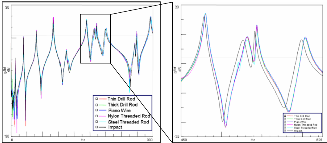
Figure 9. Stinger Type Comparison
