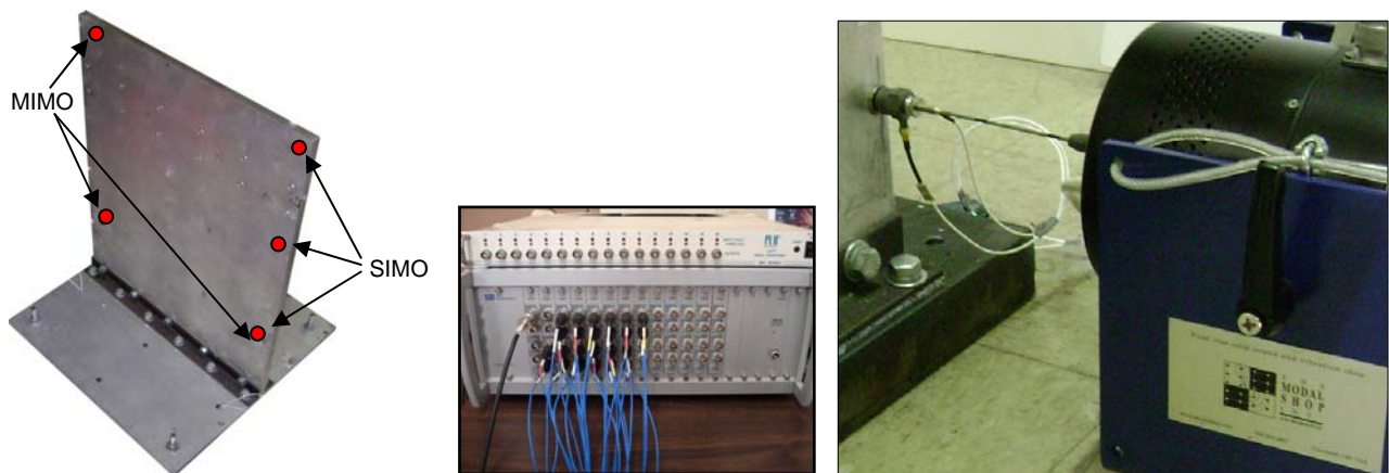
Figure 1: Base Upright Test Structure Displaying Stinger Attachment Locations and LMS SCADAS acquisition system
