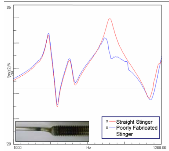
Figure 7. Poorly Fabricated Stinger Assembly
