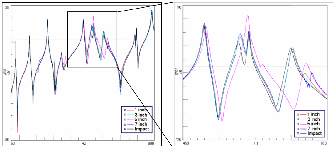
Figure 8. Stinger Length Comparisons.
