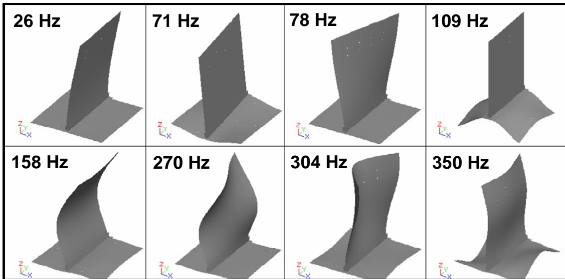
Figure 2: Typical Mode Shapes for the Test Structure.
