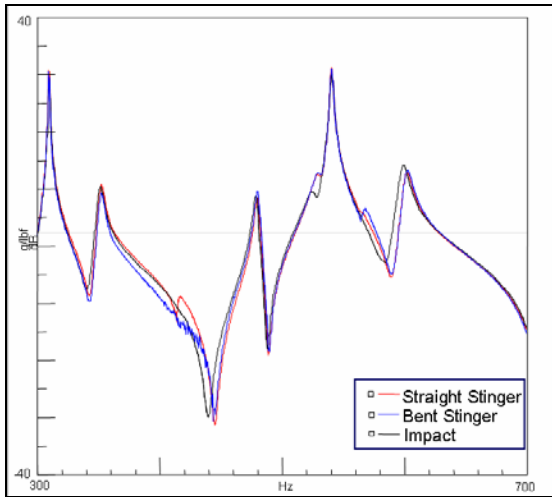
Figure 6. Intentional Stinger Misalignment
